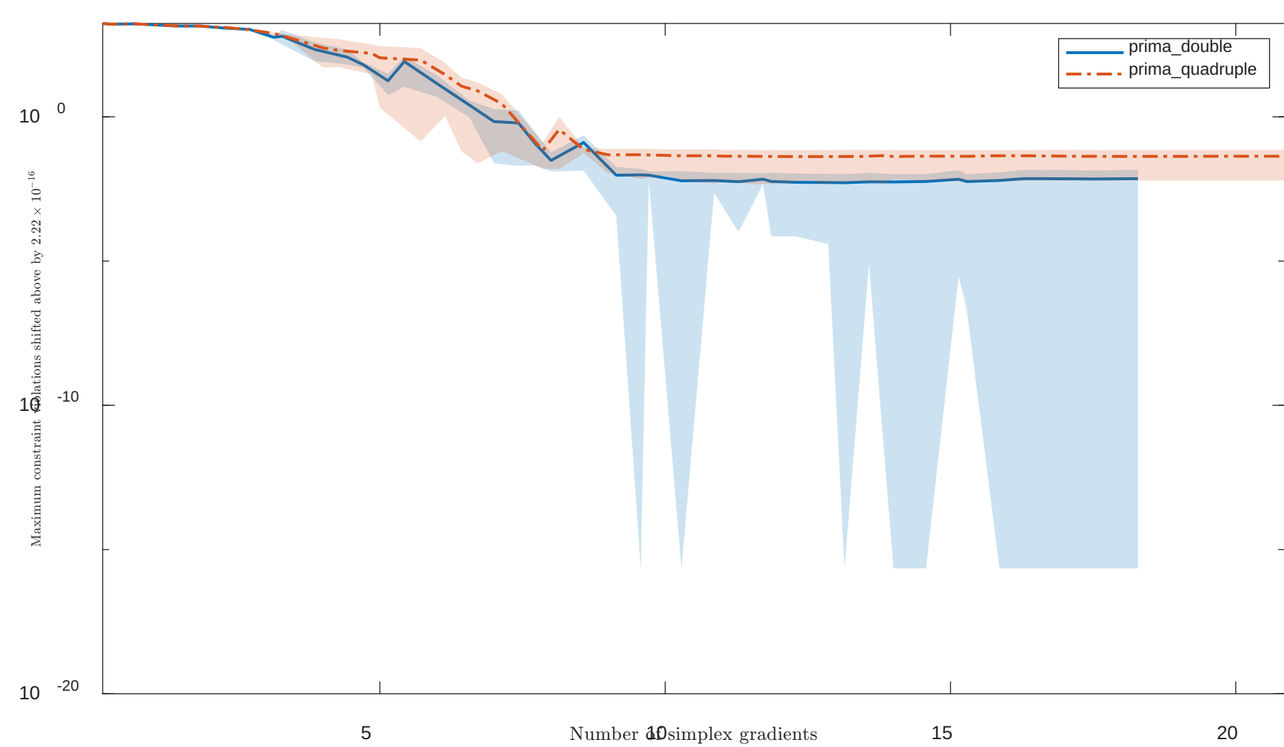
Solving “CRESC4” with “noisy” feature
