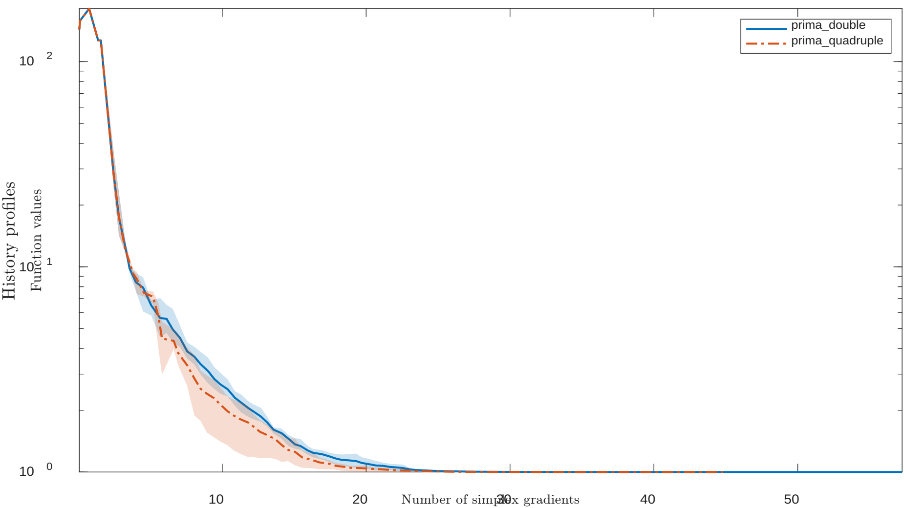
Solving "DIXMAANA1" with "noisy" feature
