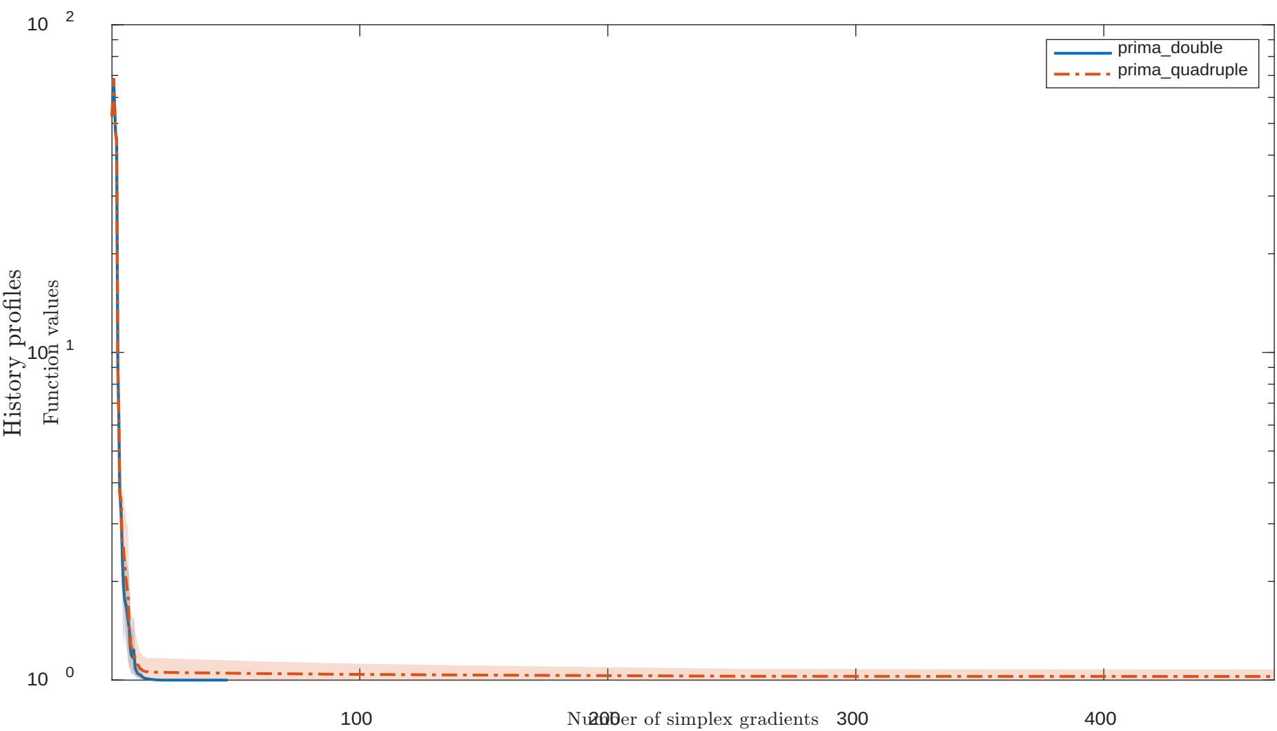
Solving “DIXMAANM1” with “noisy” feature
