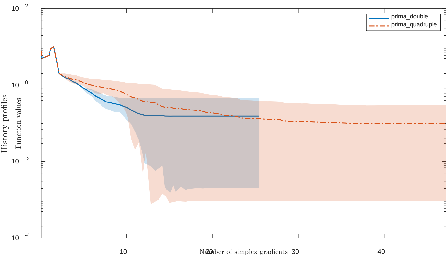
Solving "DIXON3DQ" with "noisy" feature
