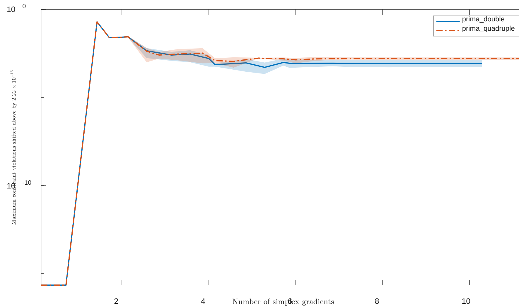
Solving "EIGENACO" with "noisy" feature
