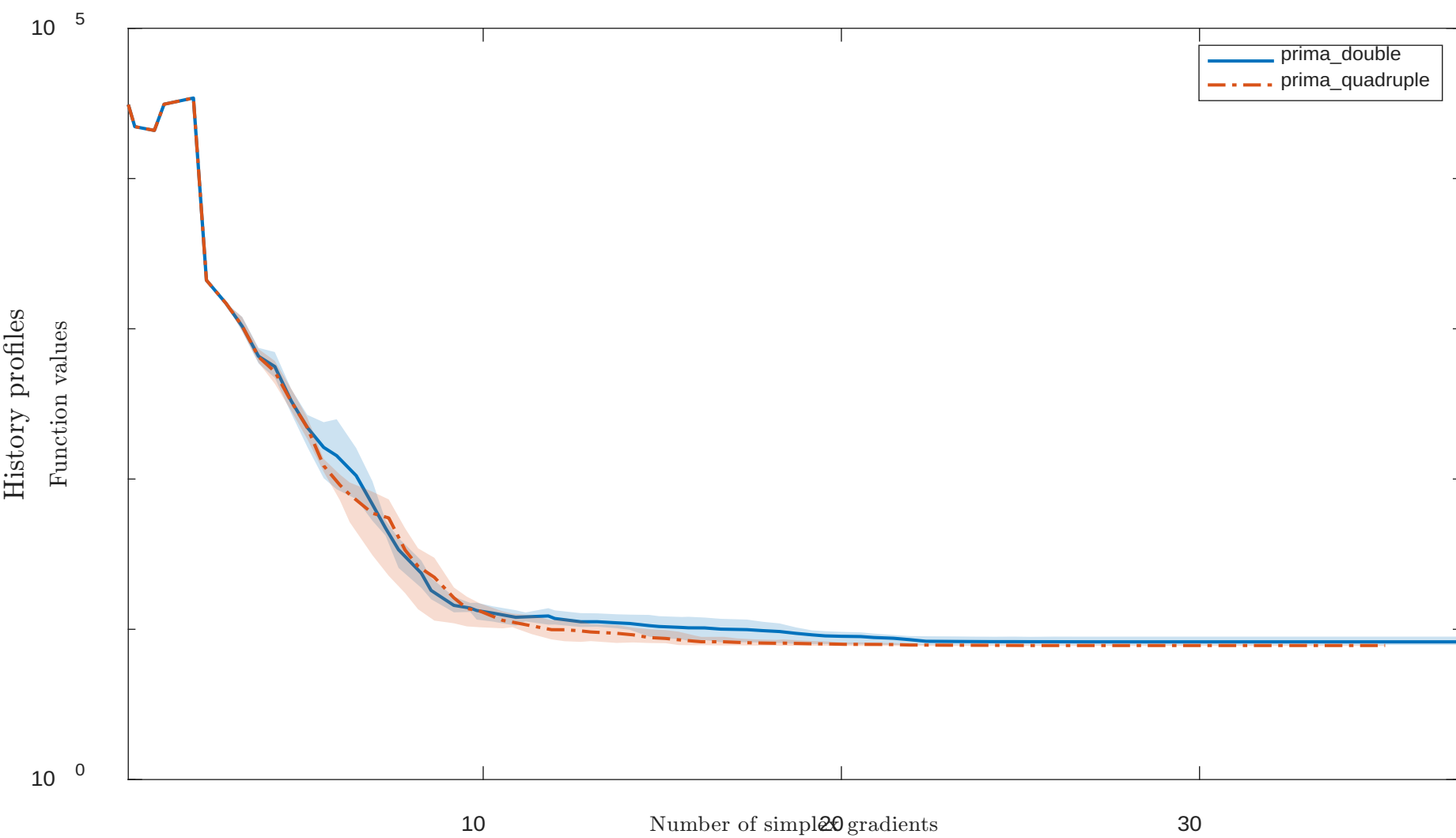
Solving “ERRINRSM” with “noisy” feature
