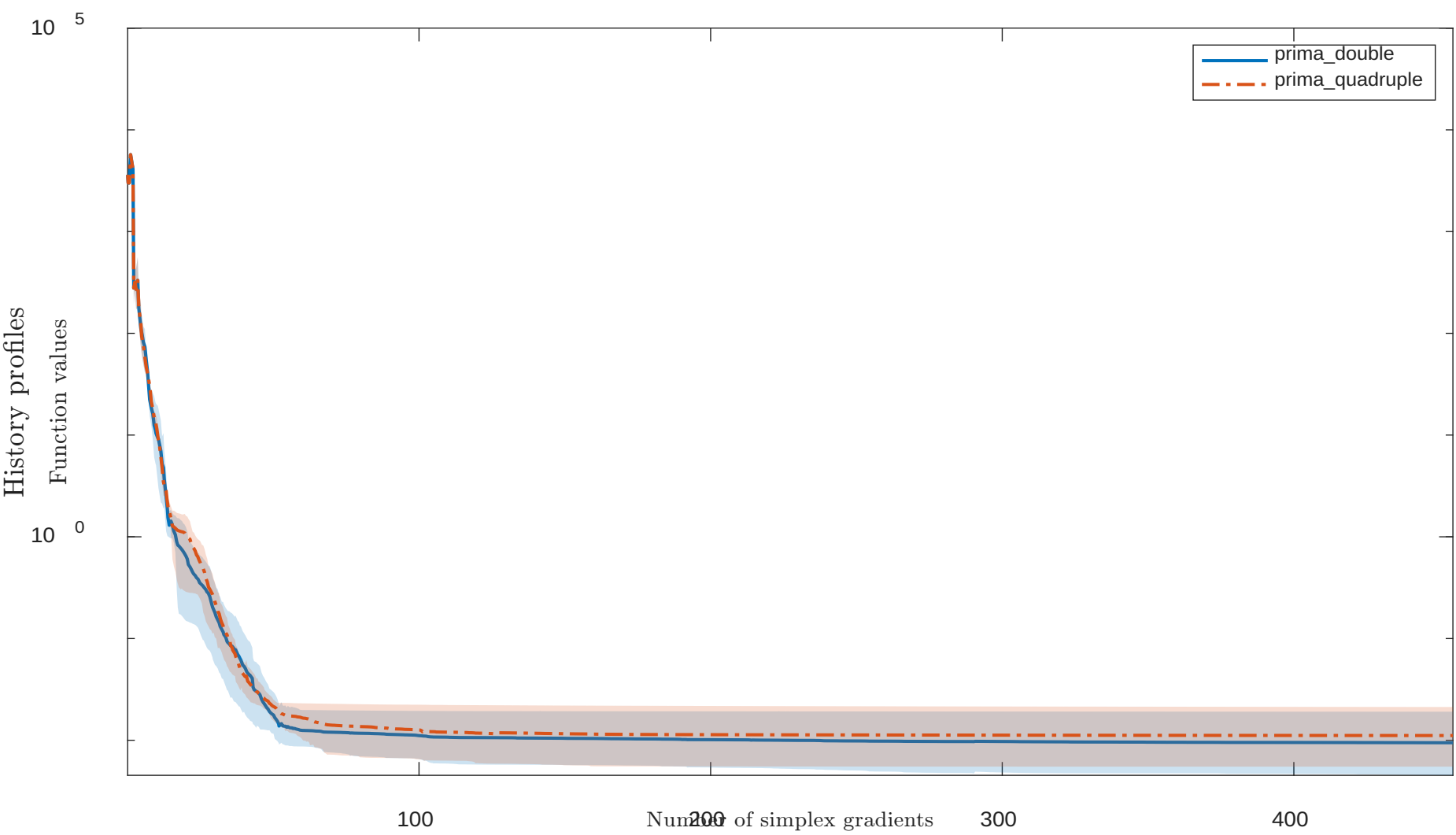
Solving “EXTROSNB” with “noisy” feature
