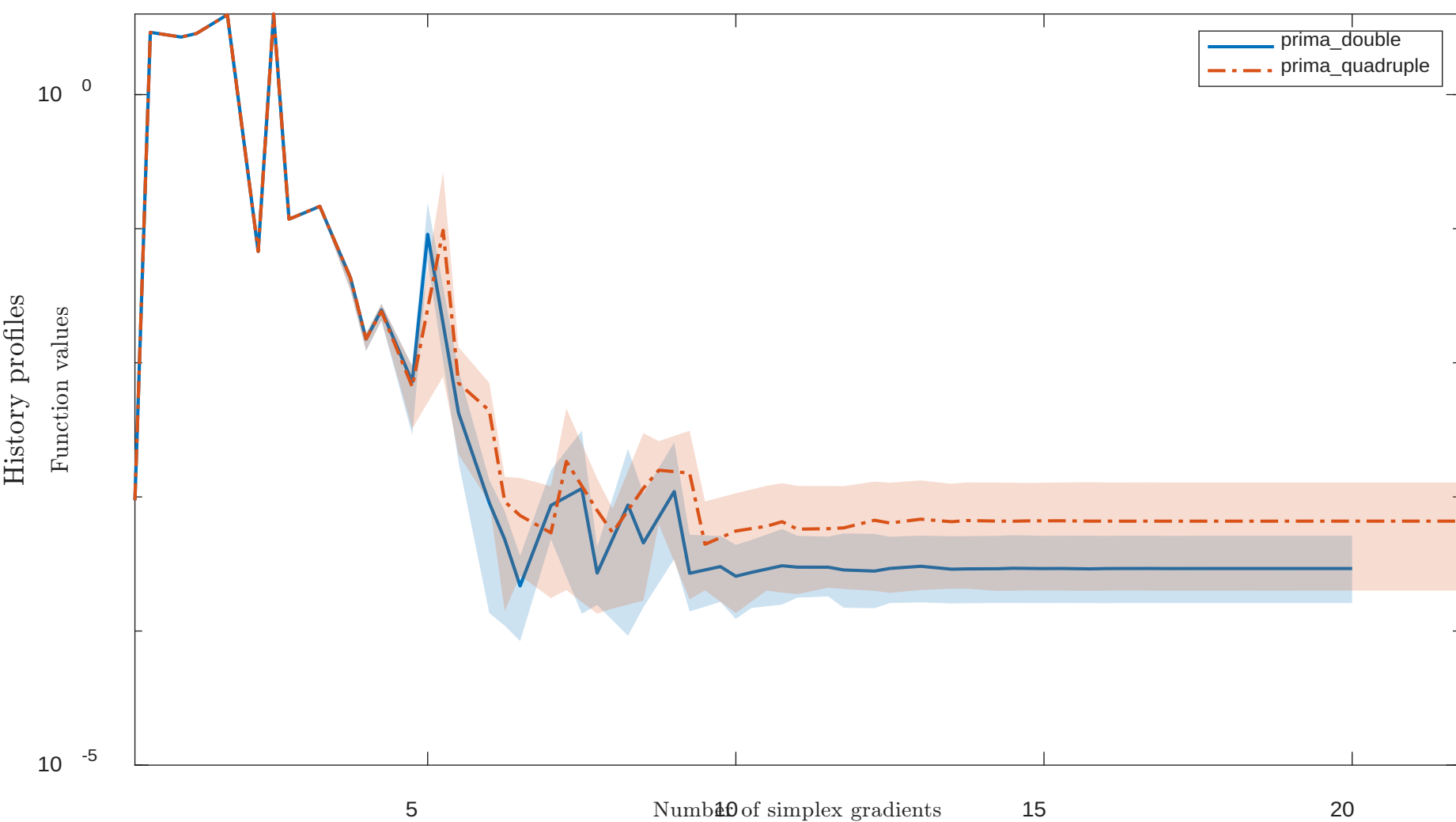
Solving “HATFLDFL” with “noisy” feature
