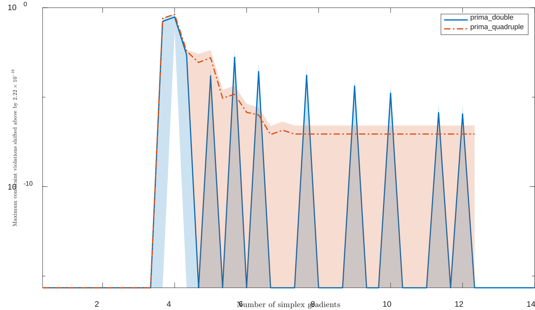
Solving "HIMMELP4" with "noisy" feature
