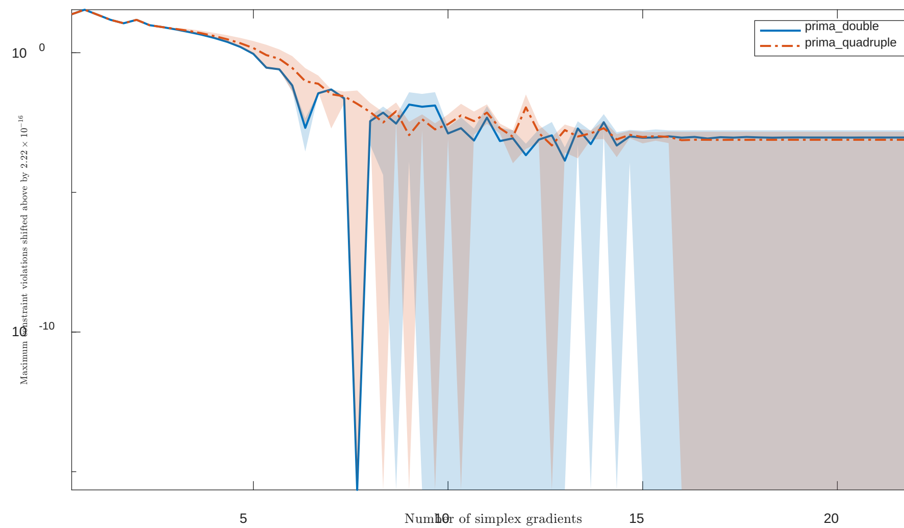
Solving "HS11" with "noisy" feature
