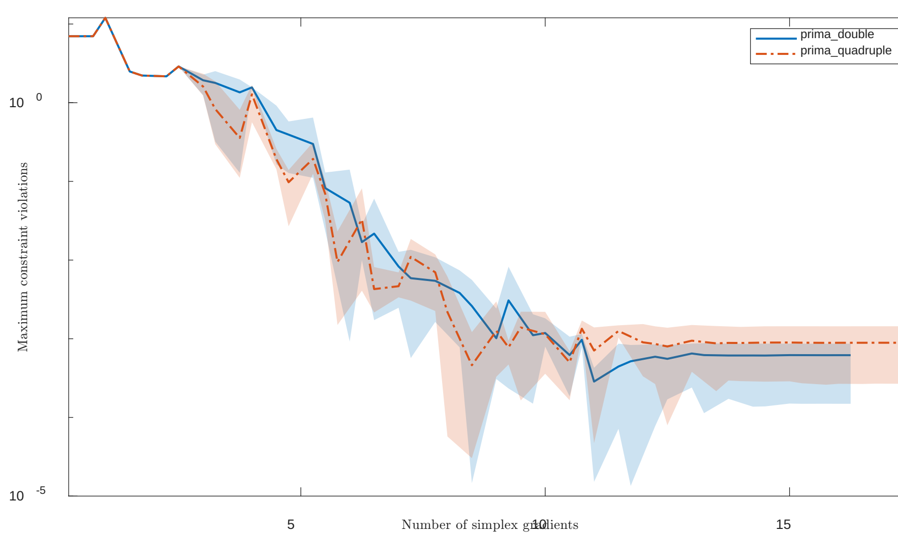
Solving "HS27" with "noisy" feature
