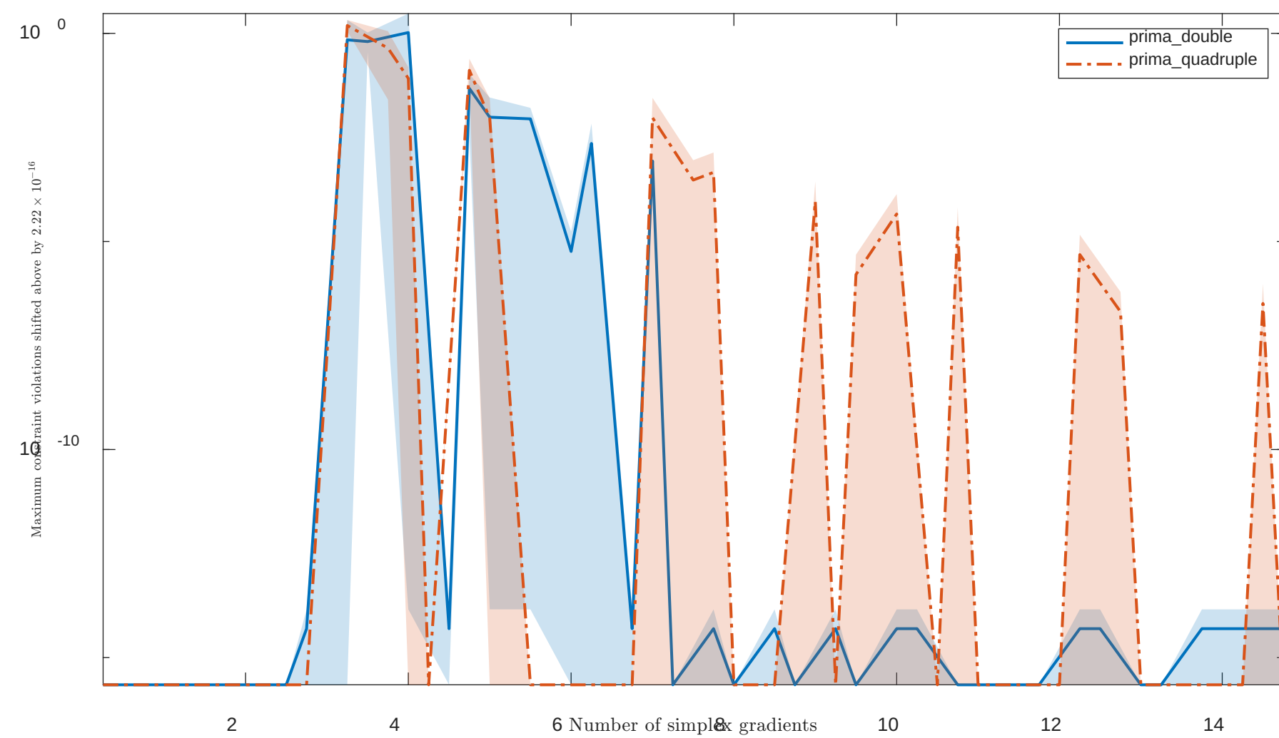
Solving "HS36" with "noisy" feature
