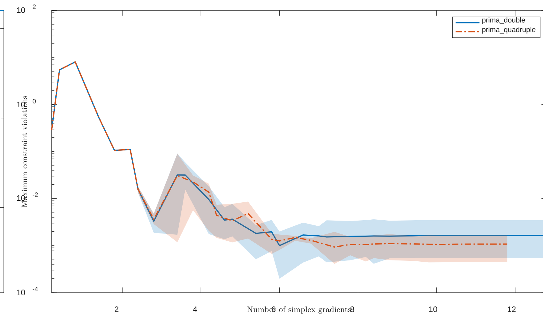
Solving "HS40" with "noisy" feature
