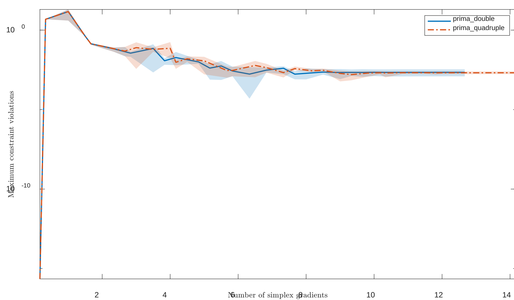
Solving "HS46" with "noisy" feature
