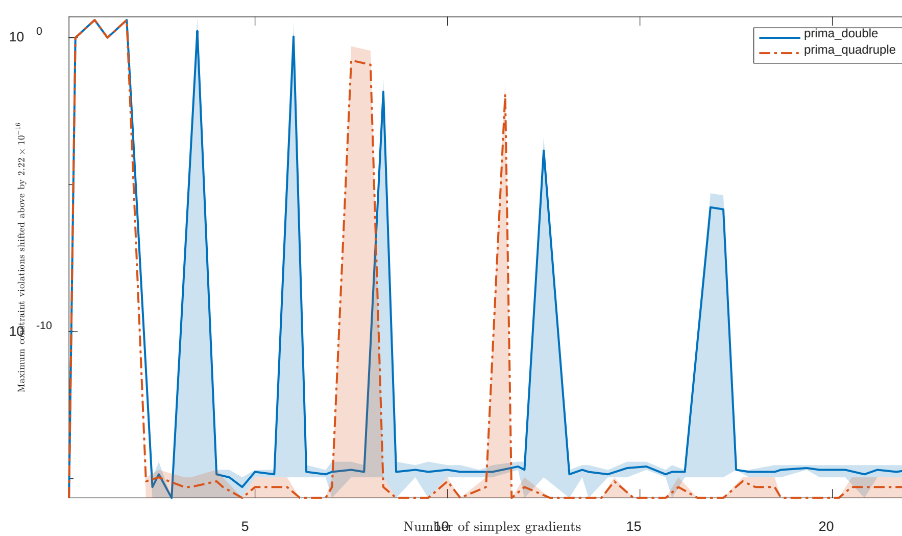
Solving "HS49" with "noisy" feature
