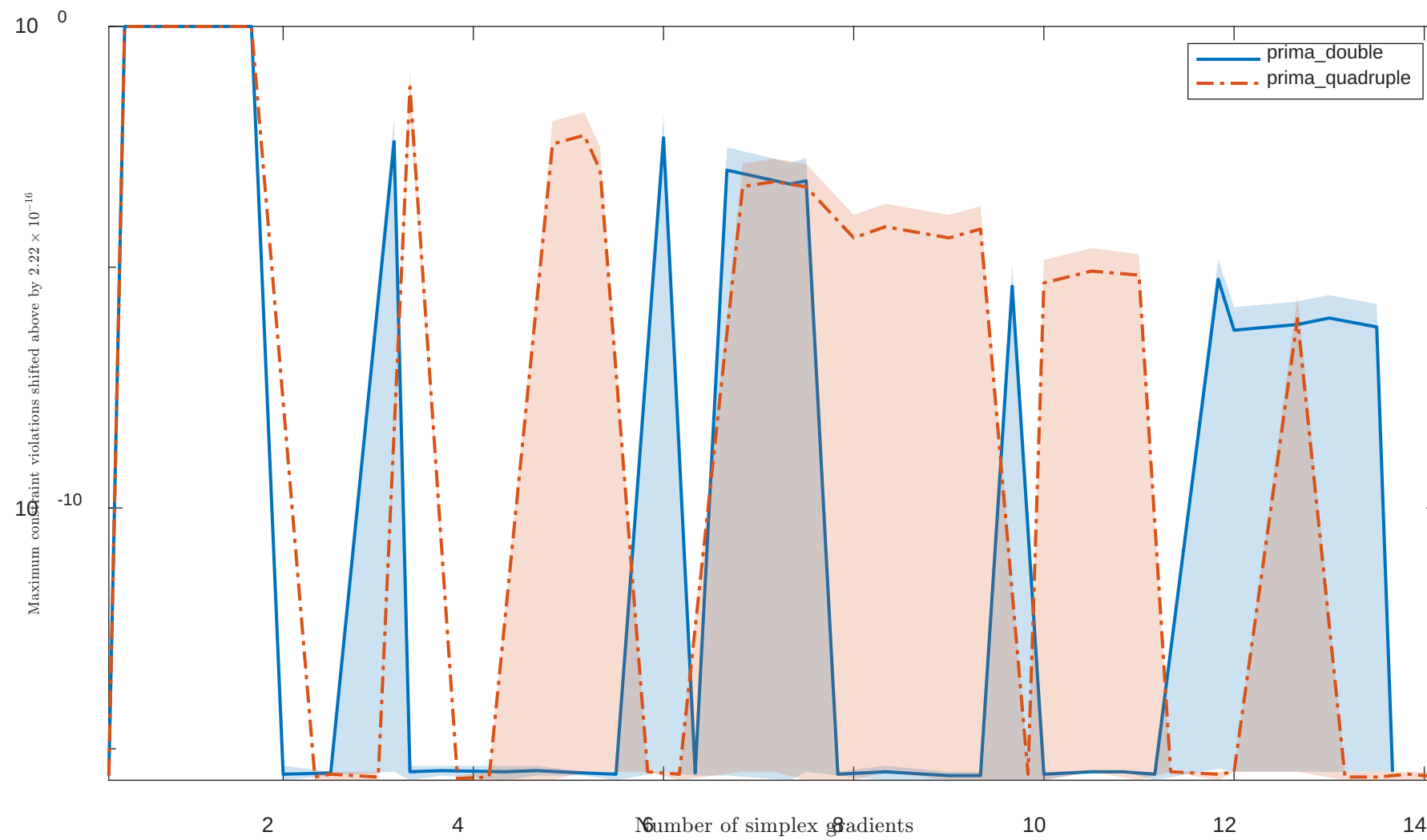
Solving “HS53” with “noisy” feature
