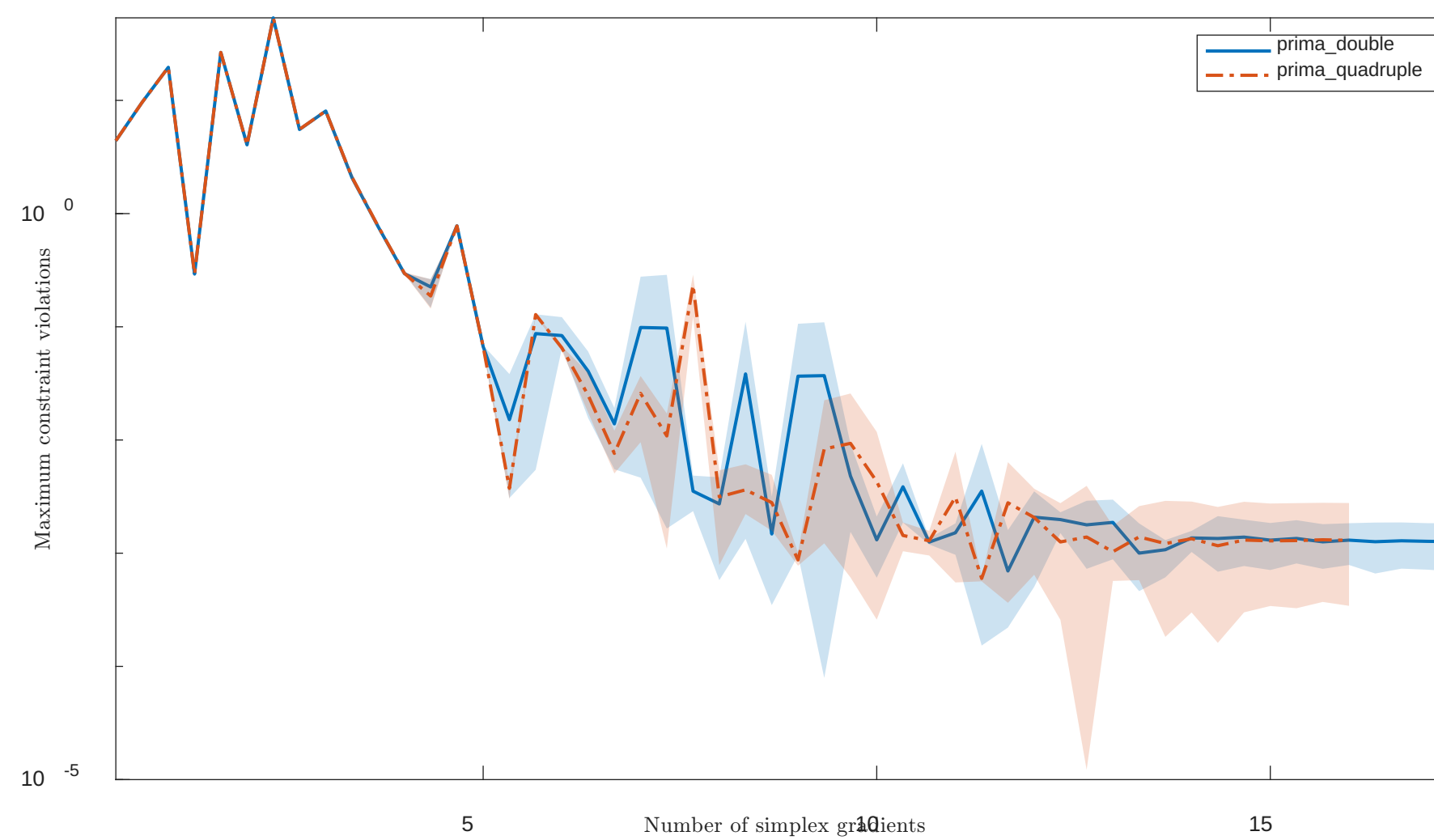
Solving "HS6" with "noisy" feature
