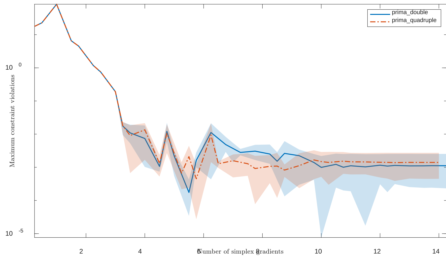
Solving "HS60" with "noisy" feature
