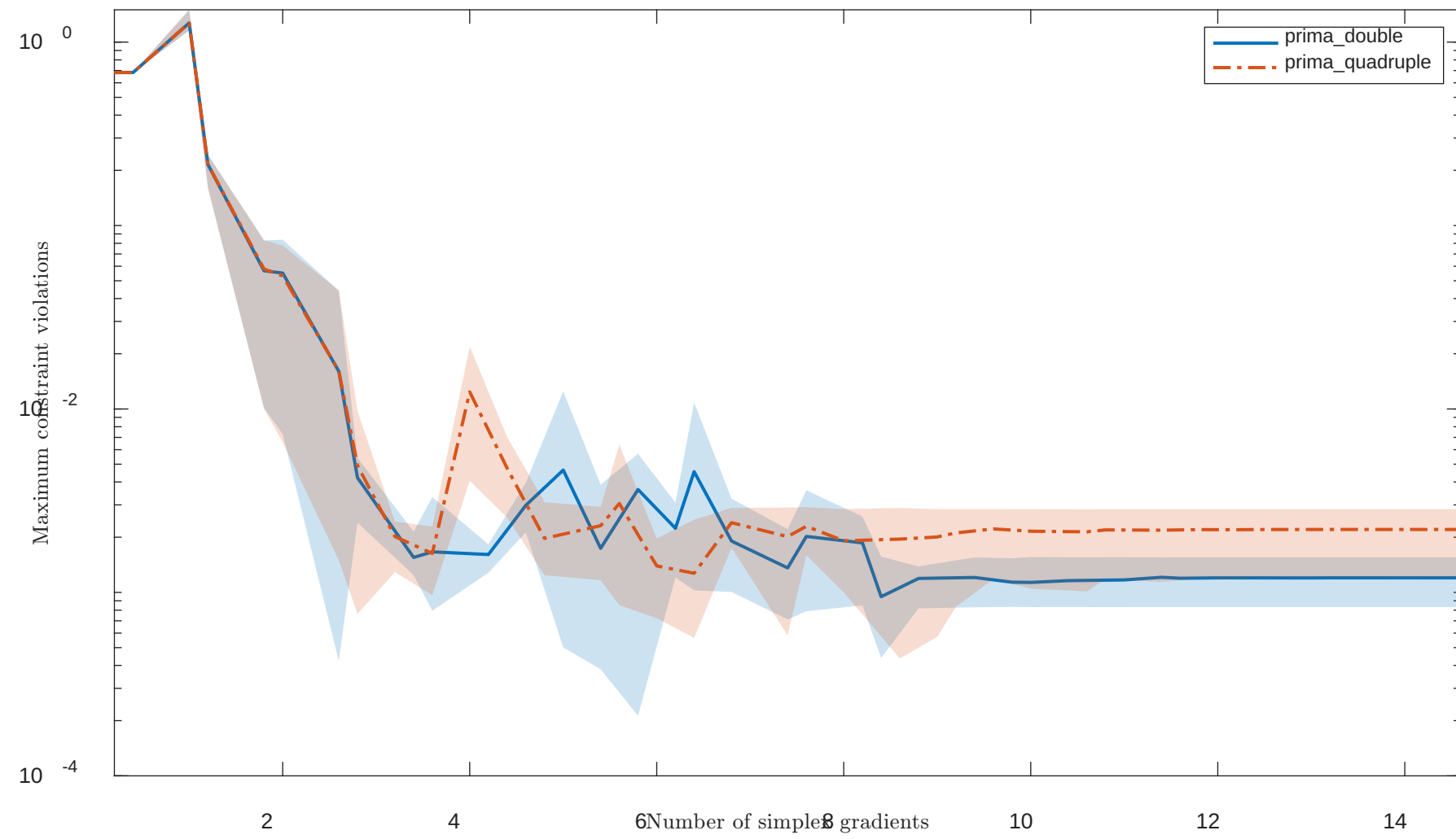
Solving “HS69” with “noisy” feature
