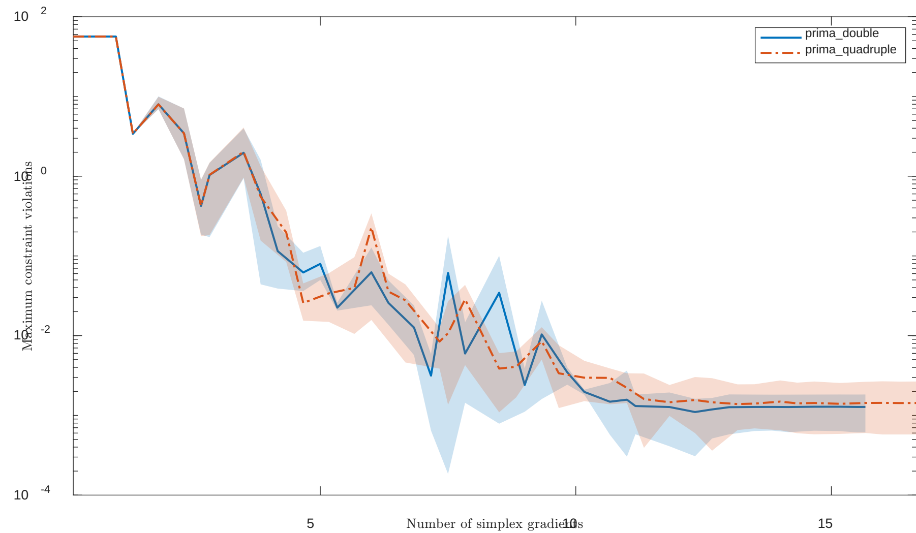
Solving "HS77" with "noisy" feature
