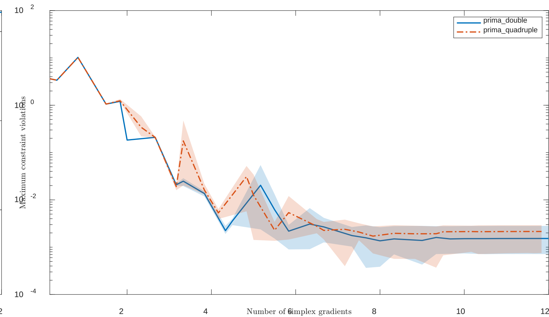
Solving "HS78" with "noisy" feature
