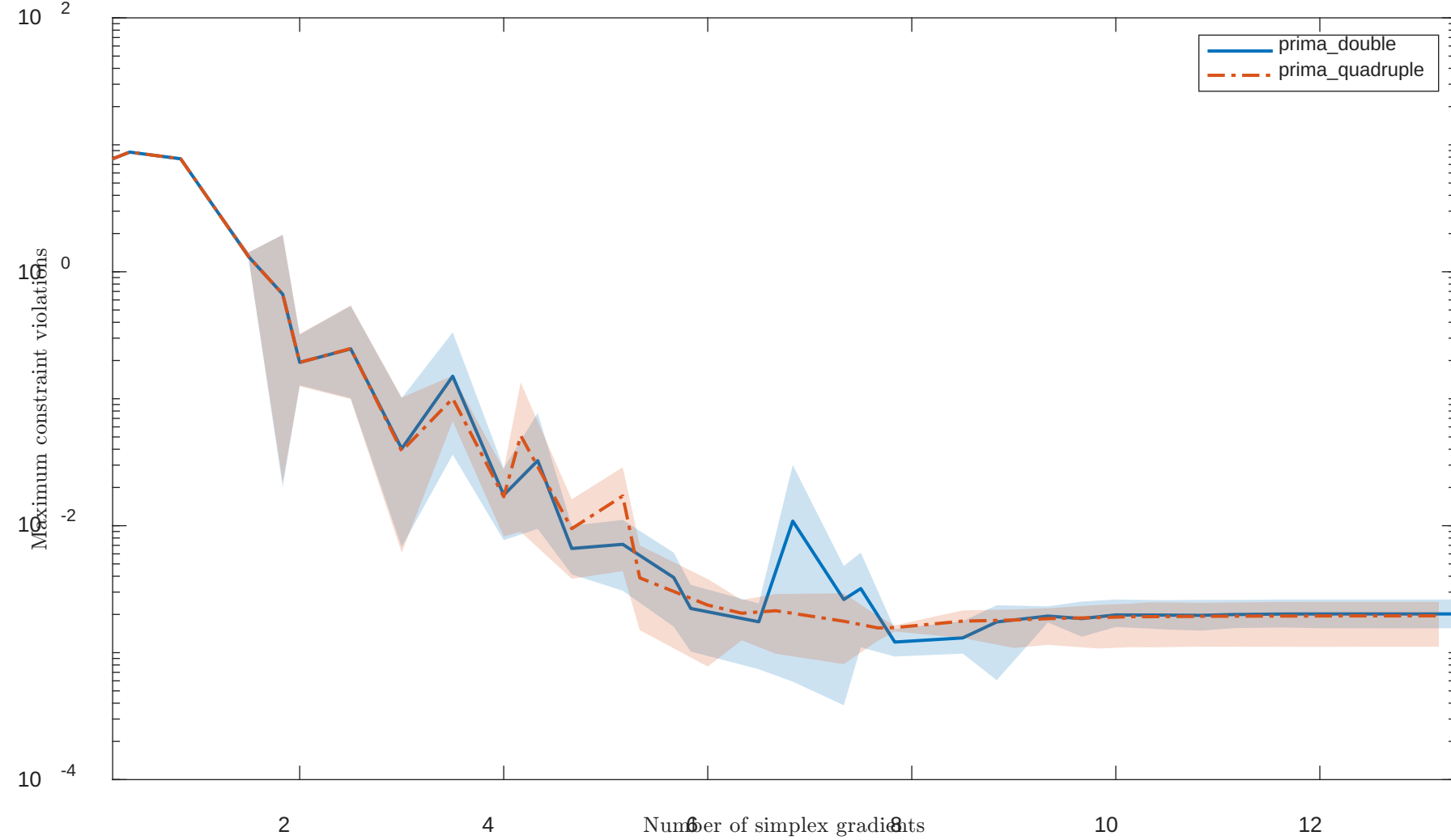
Solving "HS79" with "noisy" feature
