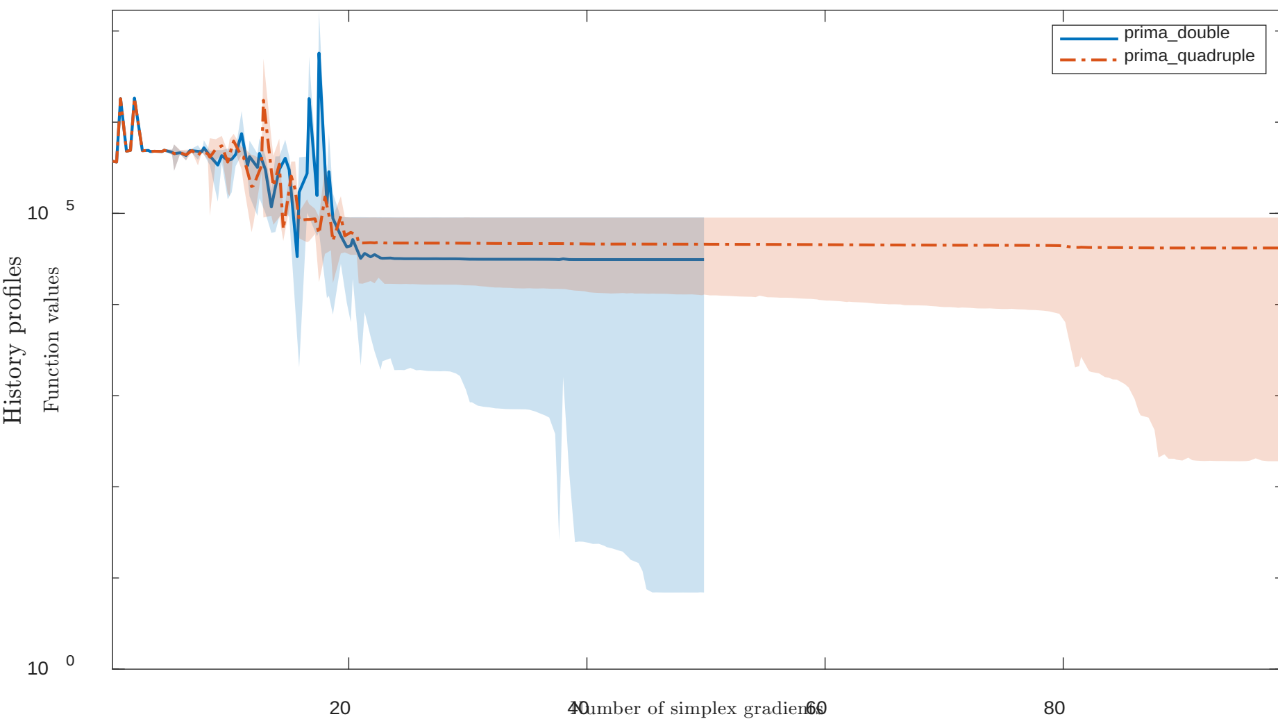
Solving “KIRBY2LS” with “noisy” feature
