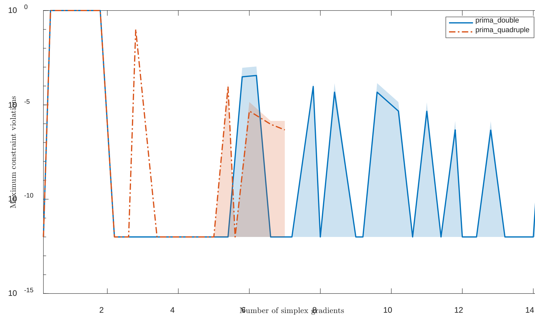
Solving "LIN" with "noisy" feature
