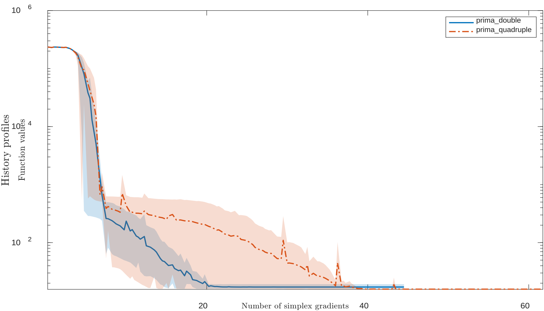
Solving “LSC2LS” with “noisy” feature
