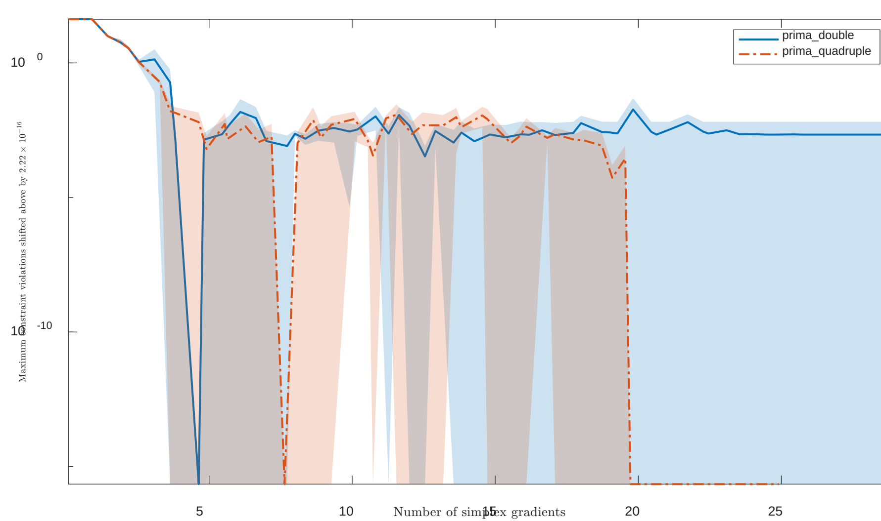
Solving "LUKVL14C" with "noisy" feature
