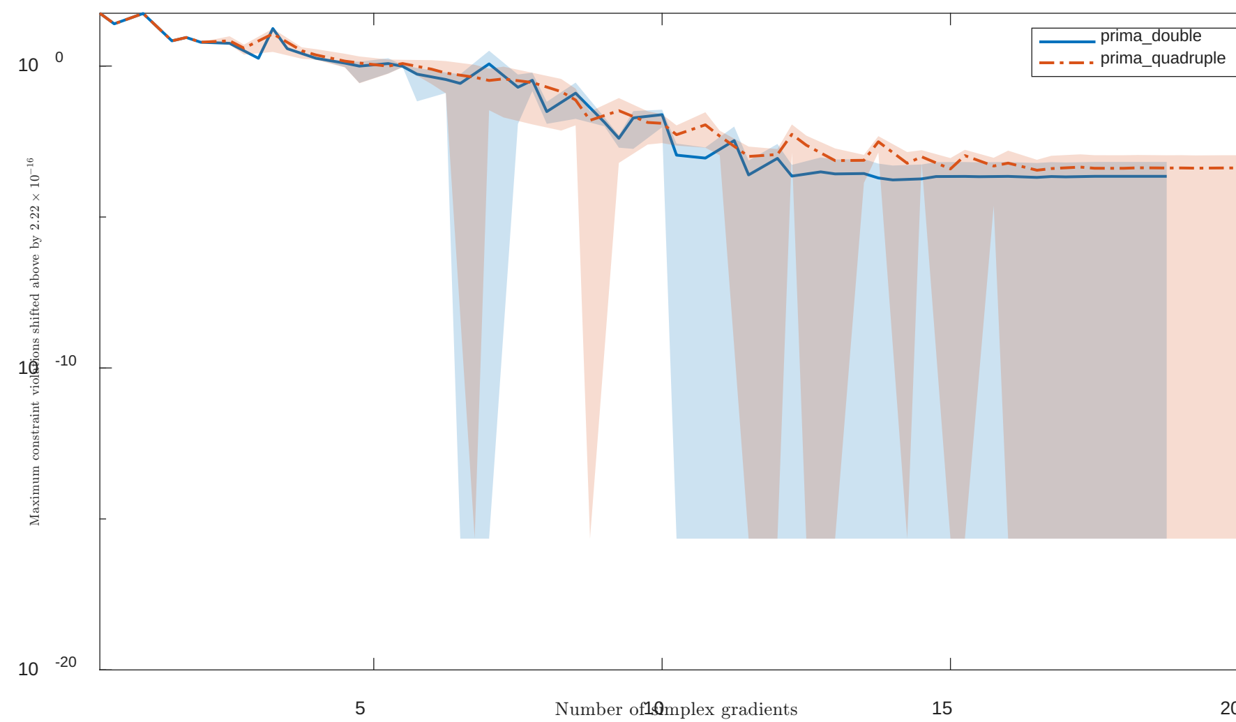
Solving “MAKELA2” with “noisy” feature
