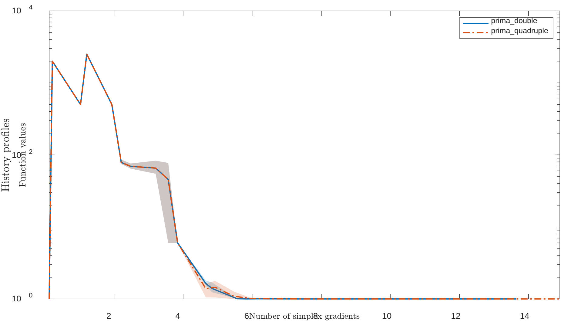
Solving “OSCIPATH” with “noisy” feature
