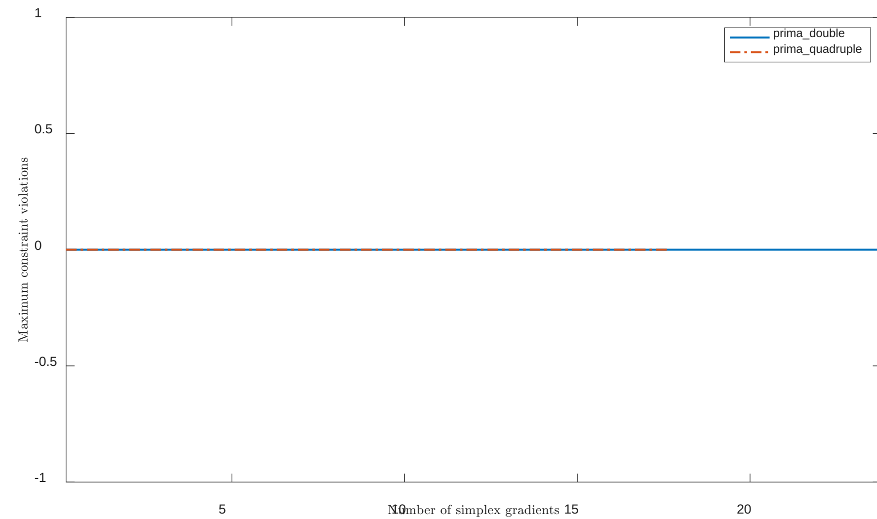
Solving "PALMER4" with "noisy" feature
