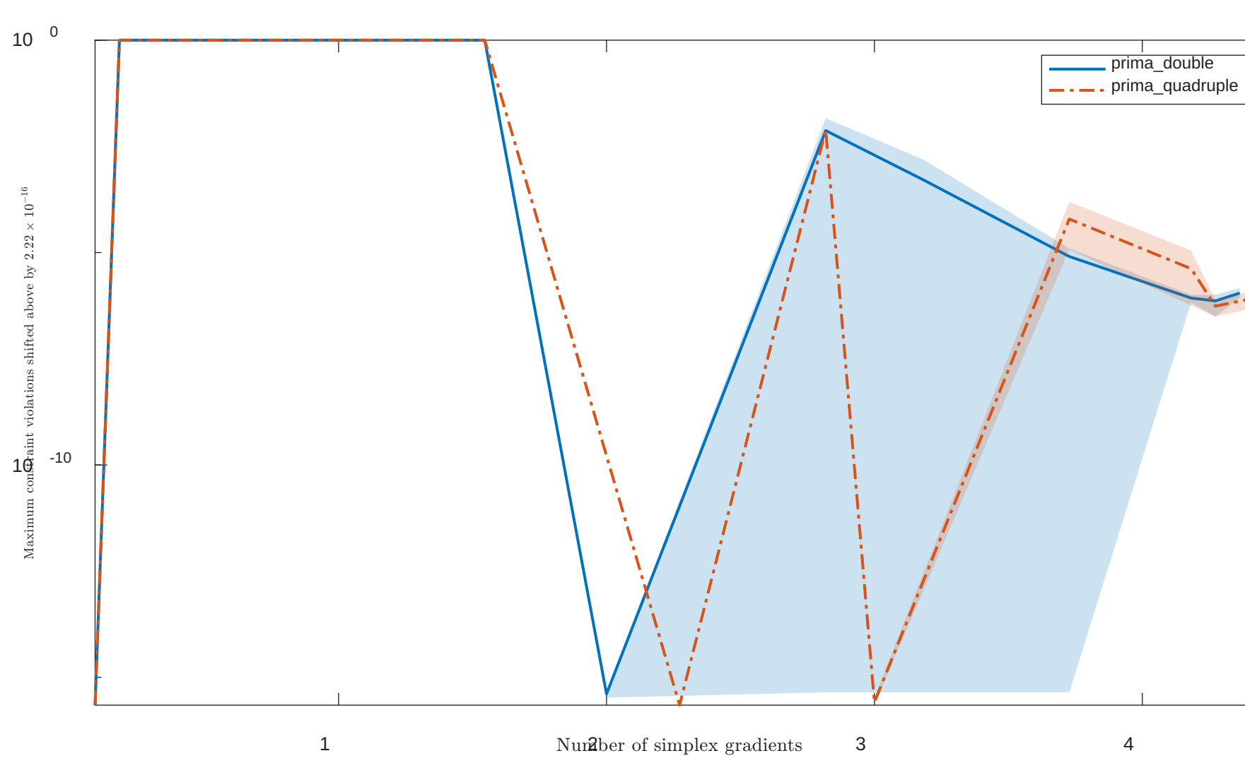
Solving "PORTSNQP" with "noisy" feature
