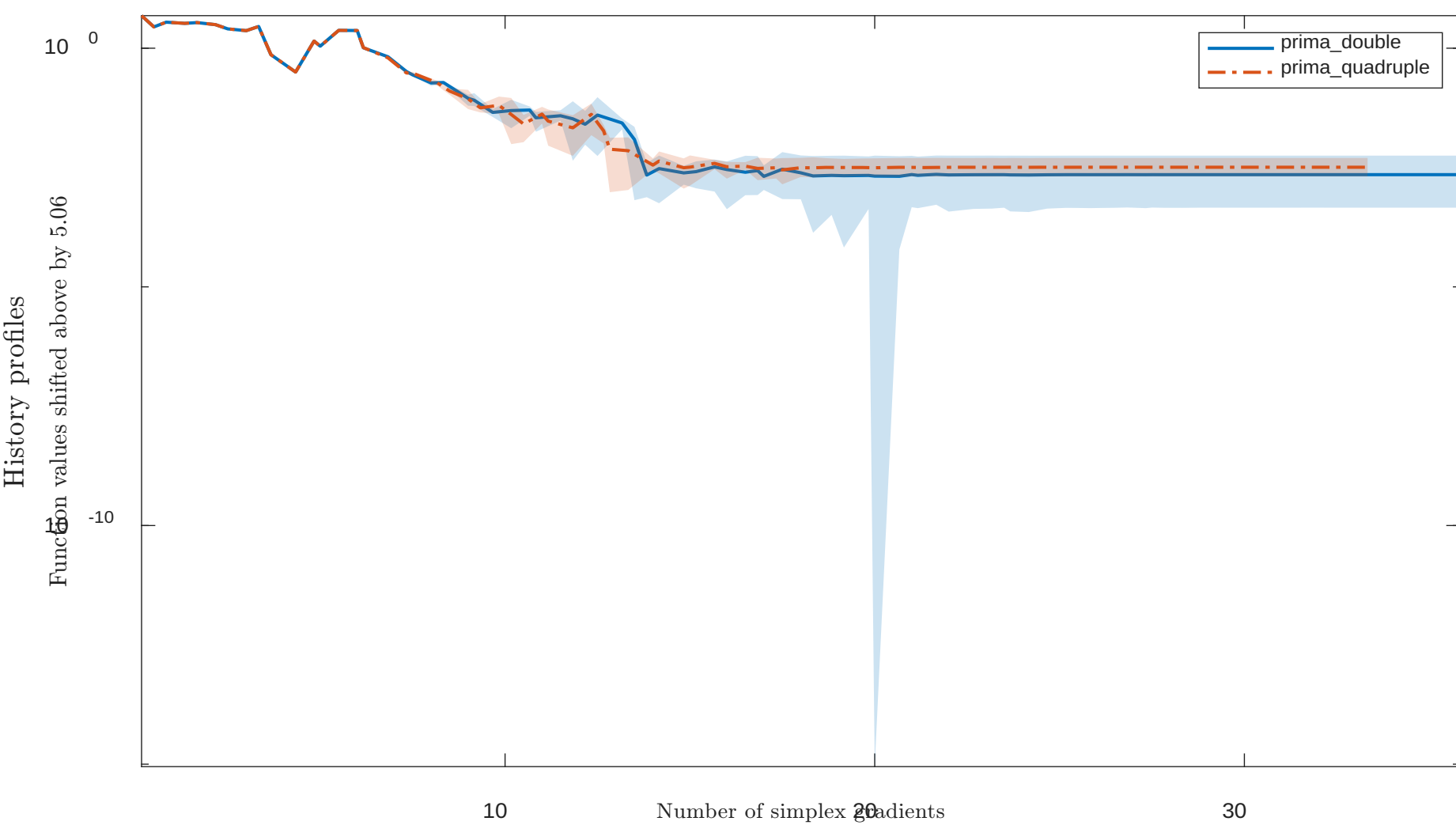
Solving “SENSORS” with “noisy” feature
