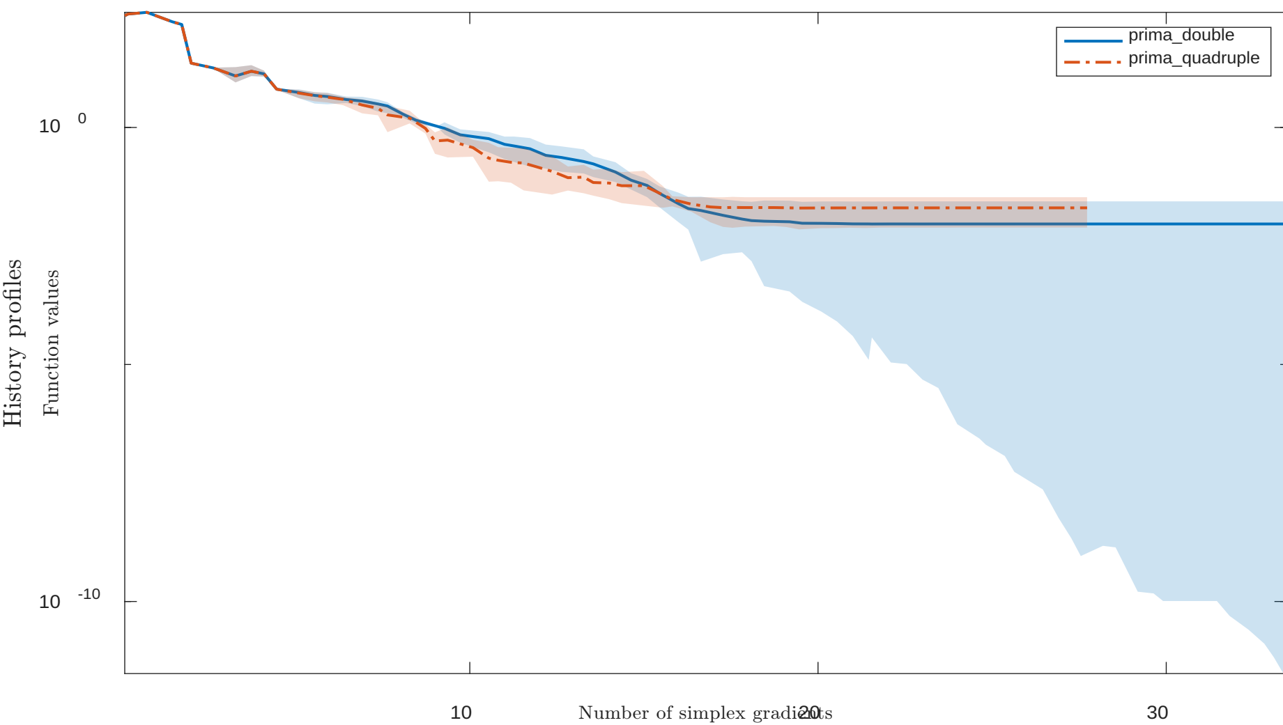
Solving “SPARSINE” with “noisy” feature
