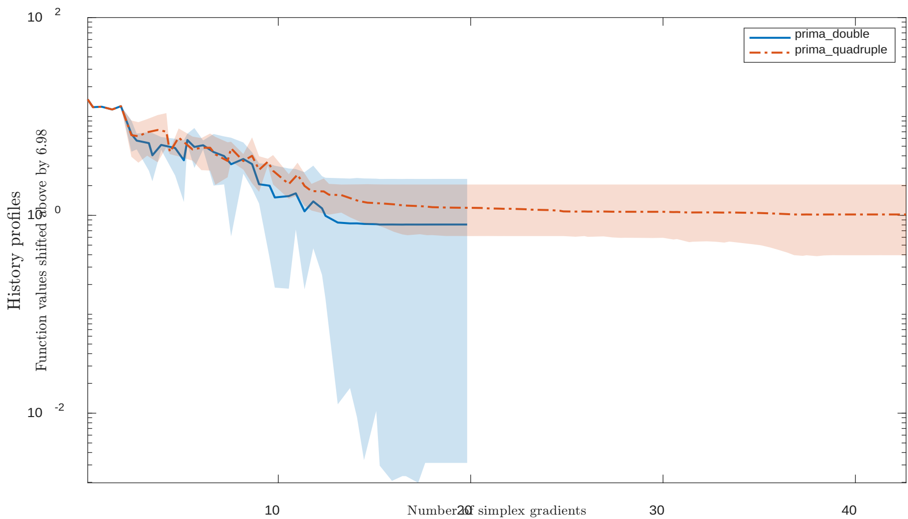
Solving “SSCOSINE” with “noisy” feature
