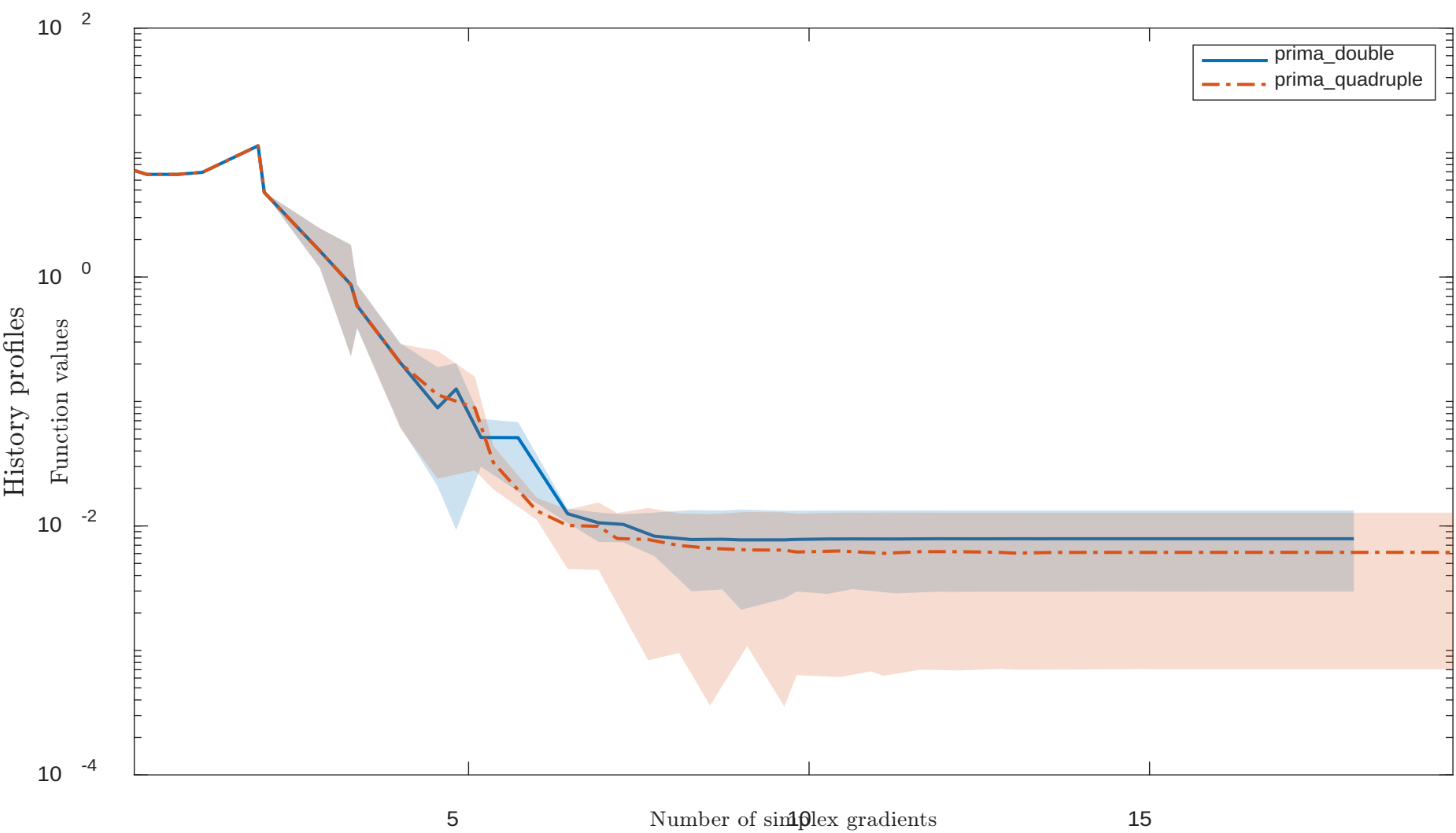
Solving "STRTCHDV" with "noisy" feature
