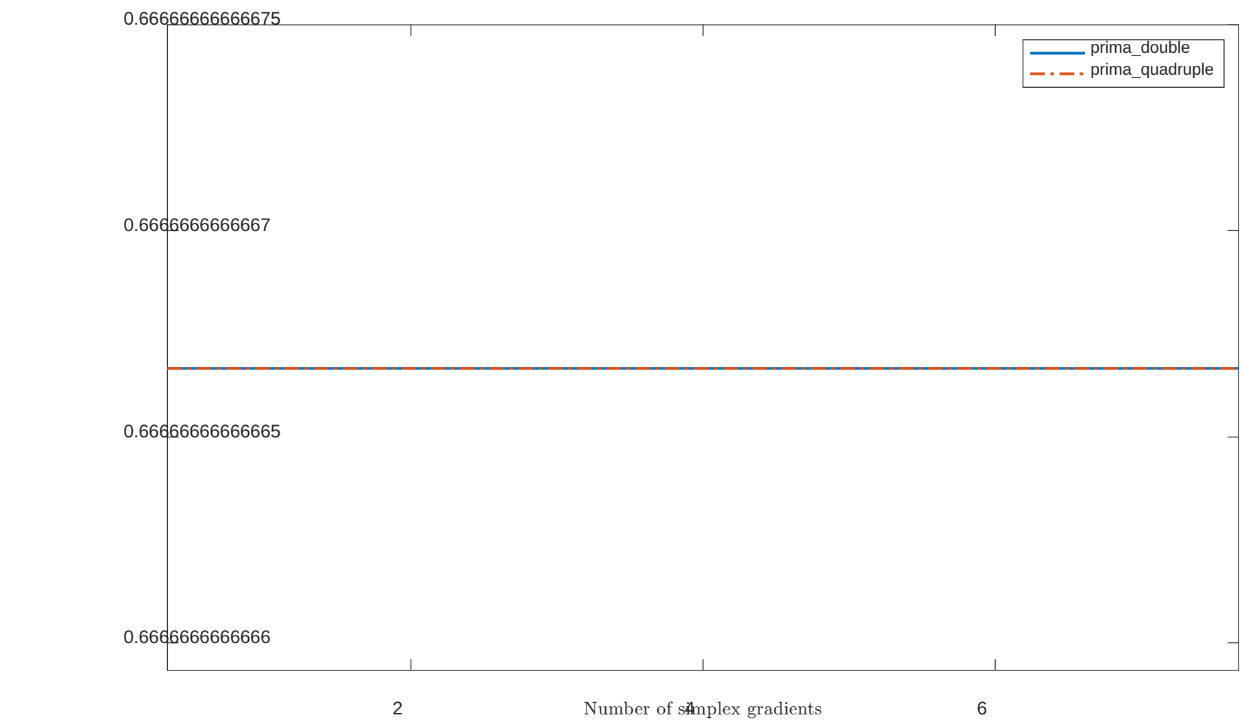
Cummin of merit function values
