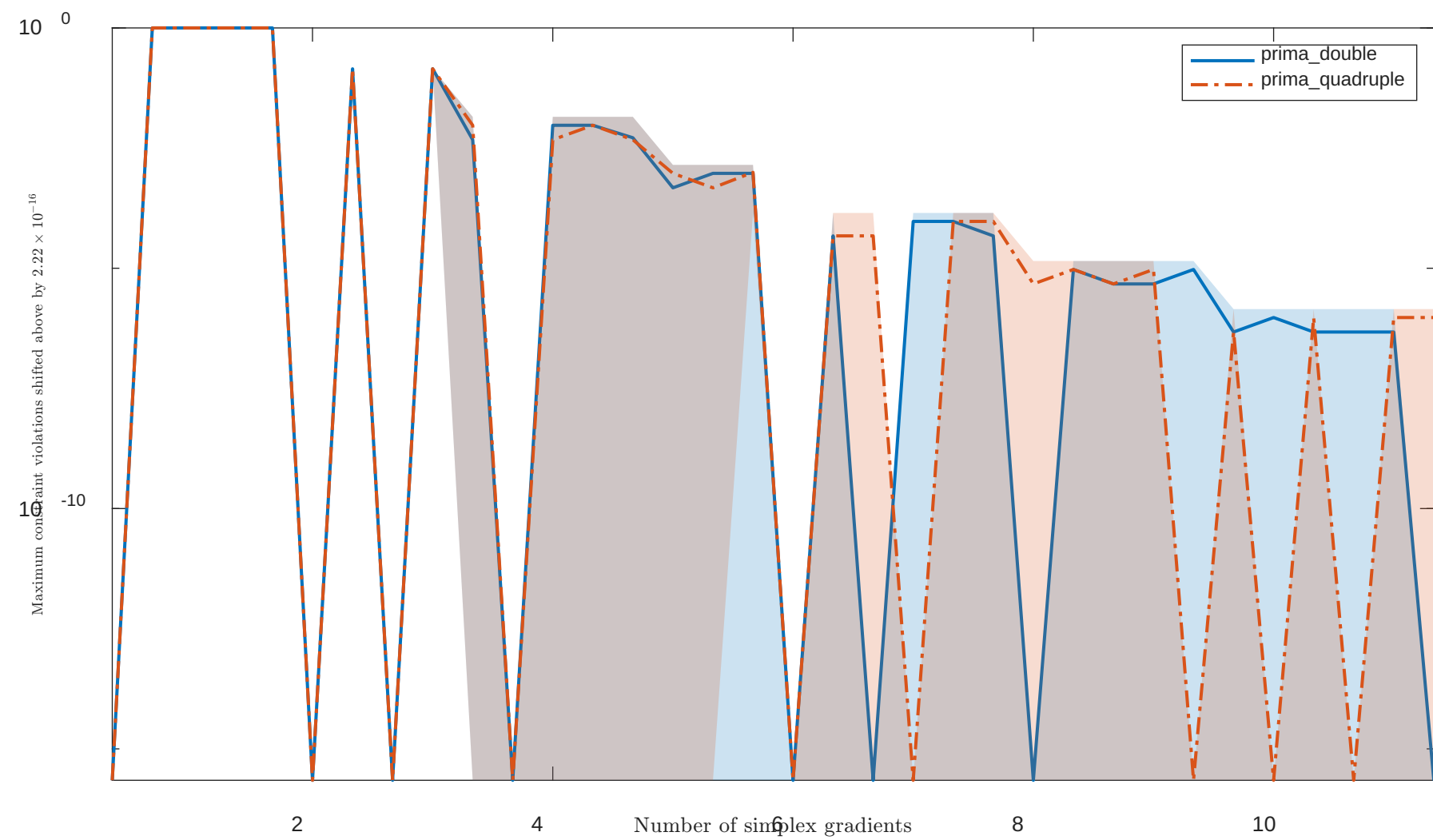
Solving “TAME” with “noisy” feature
