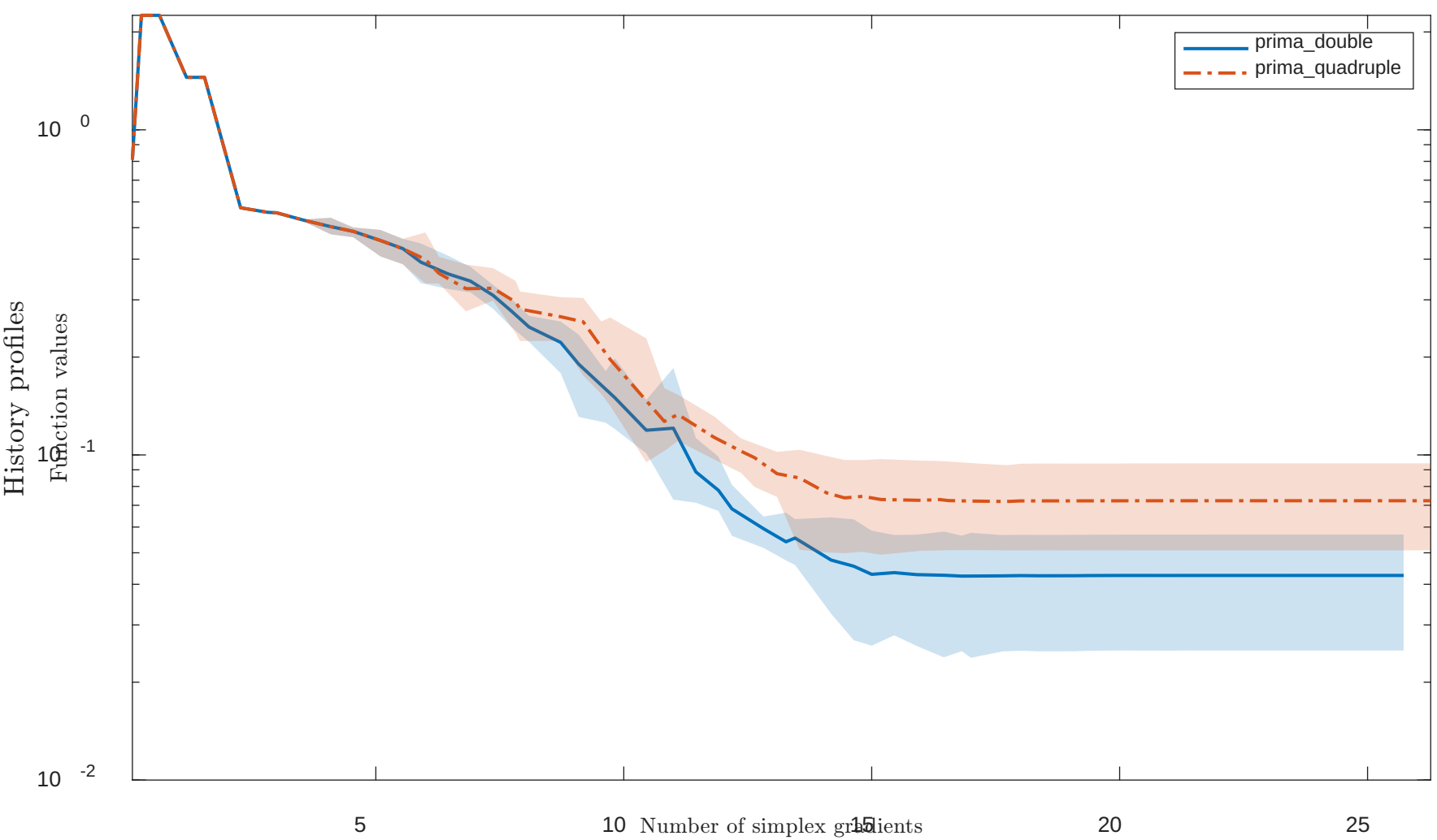
Solving “TQUARTIC” with “noisy” feature
