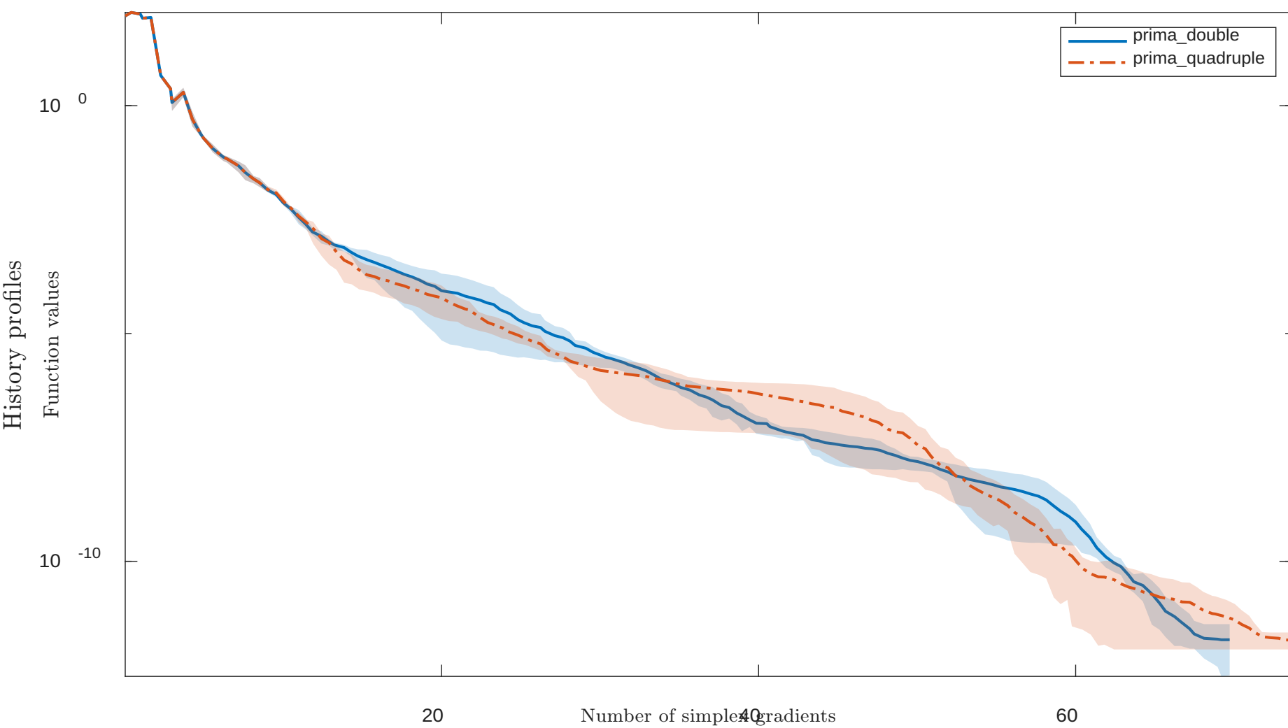
Solving “VAREIGVL” with “noisy” feature
