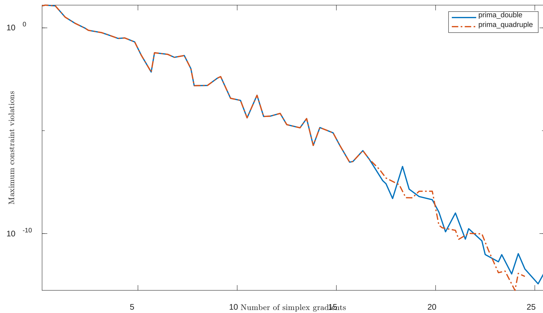
Solving "BT11" with "plain" feature
