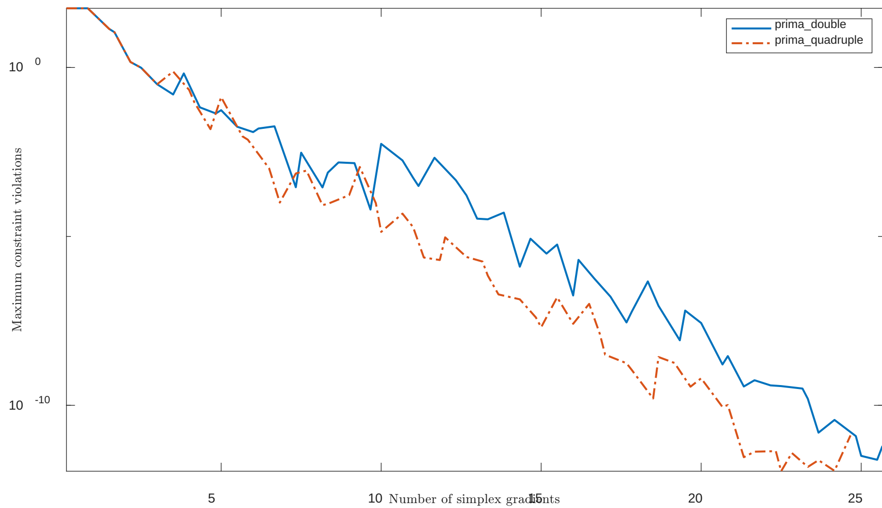
Solving "BT6" with "plain" feature
