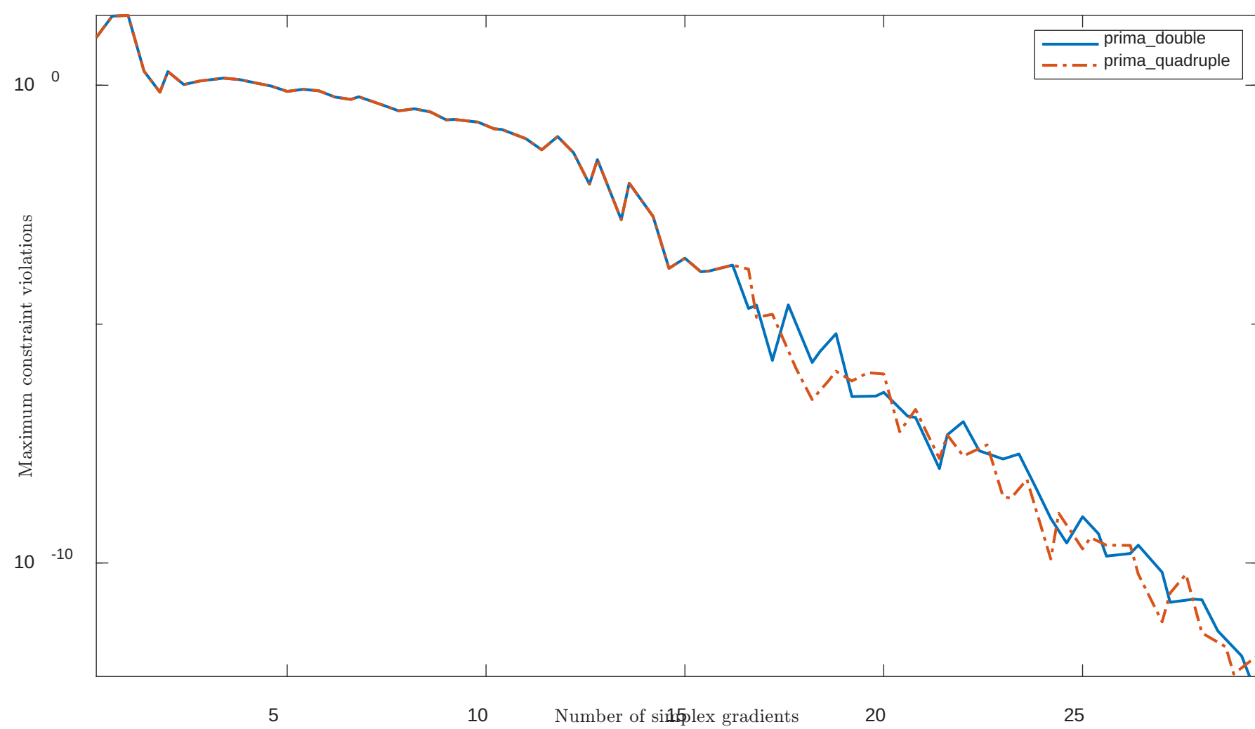
Solving "BT9" with "plain" feature
