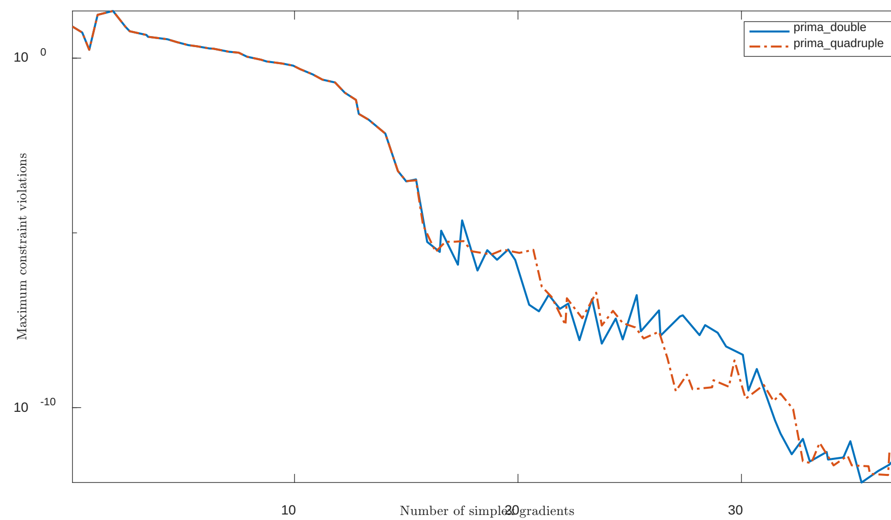
Solving “CATENARY” with “plain” feature
