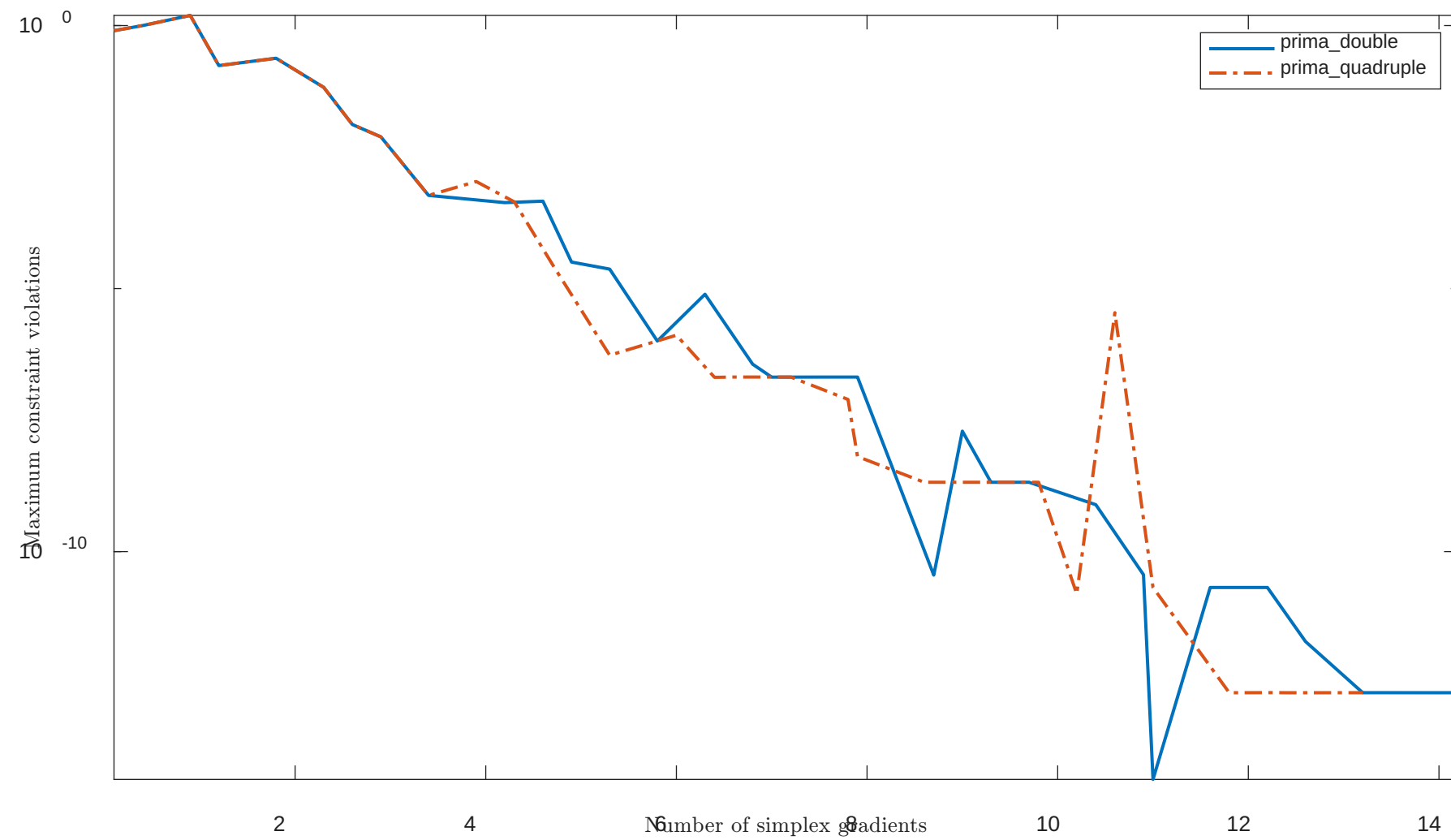
Solving "HS107" with "plain" feature
