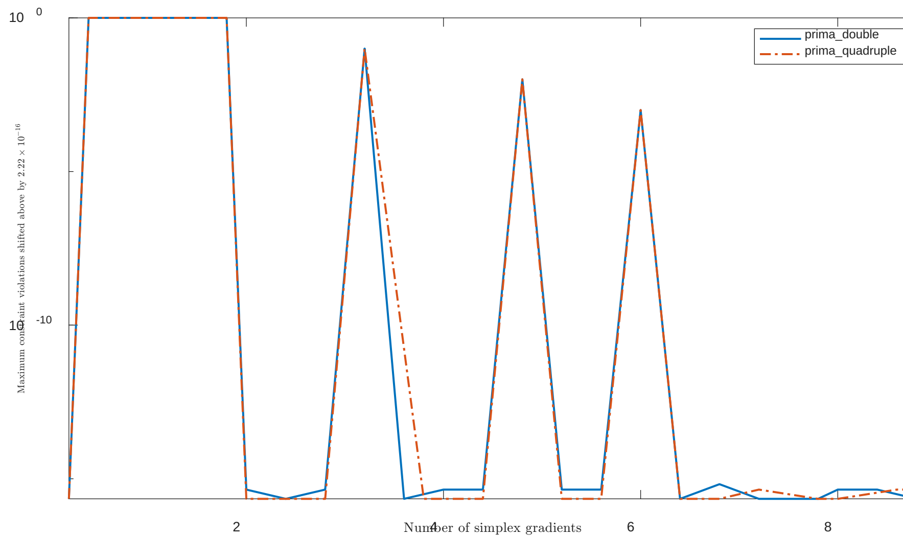
Solving “HS41” with “plain” feature
