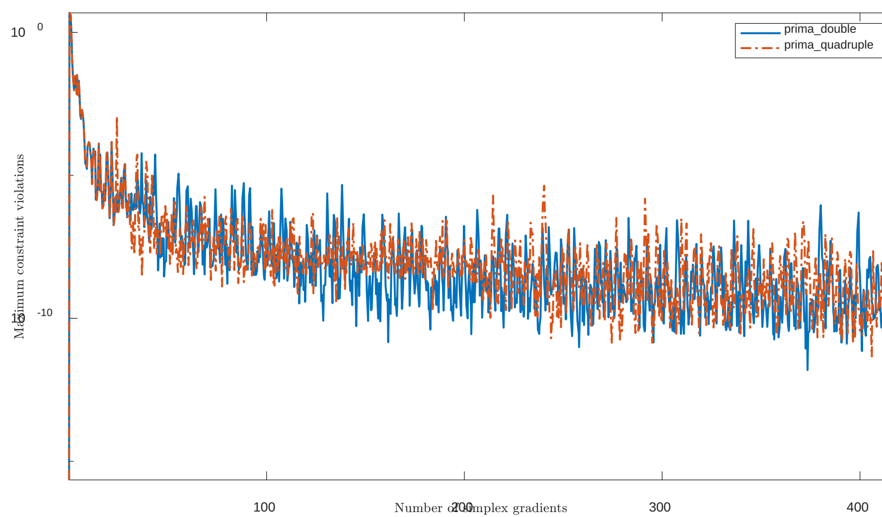
Solving "HS46" with "plain" feature
