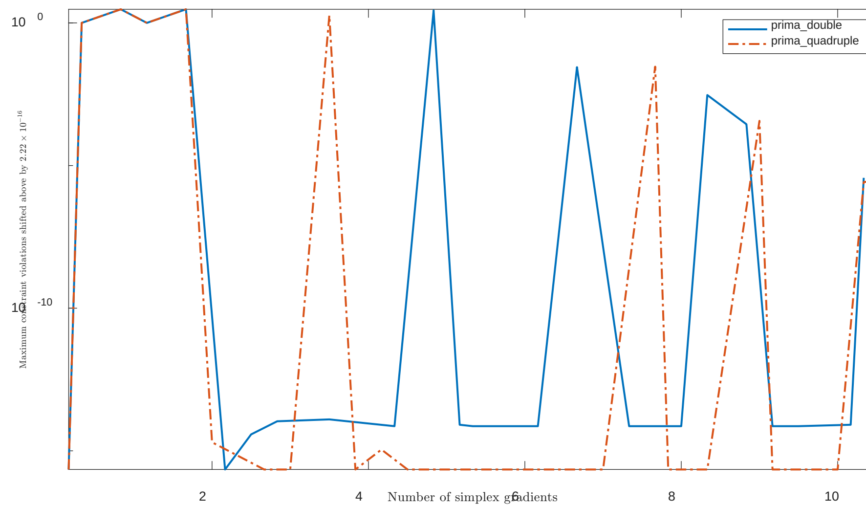
Solving "HS50" with "plain" feature
