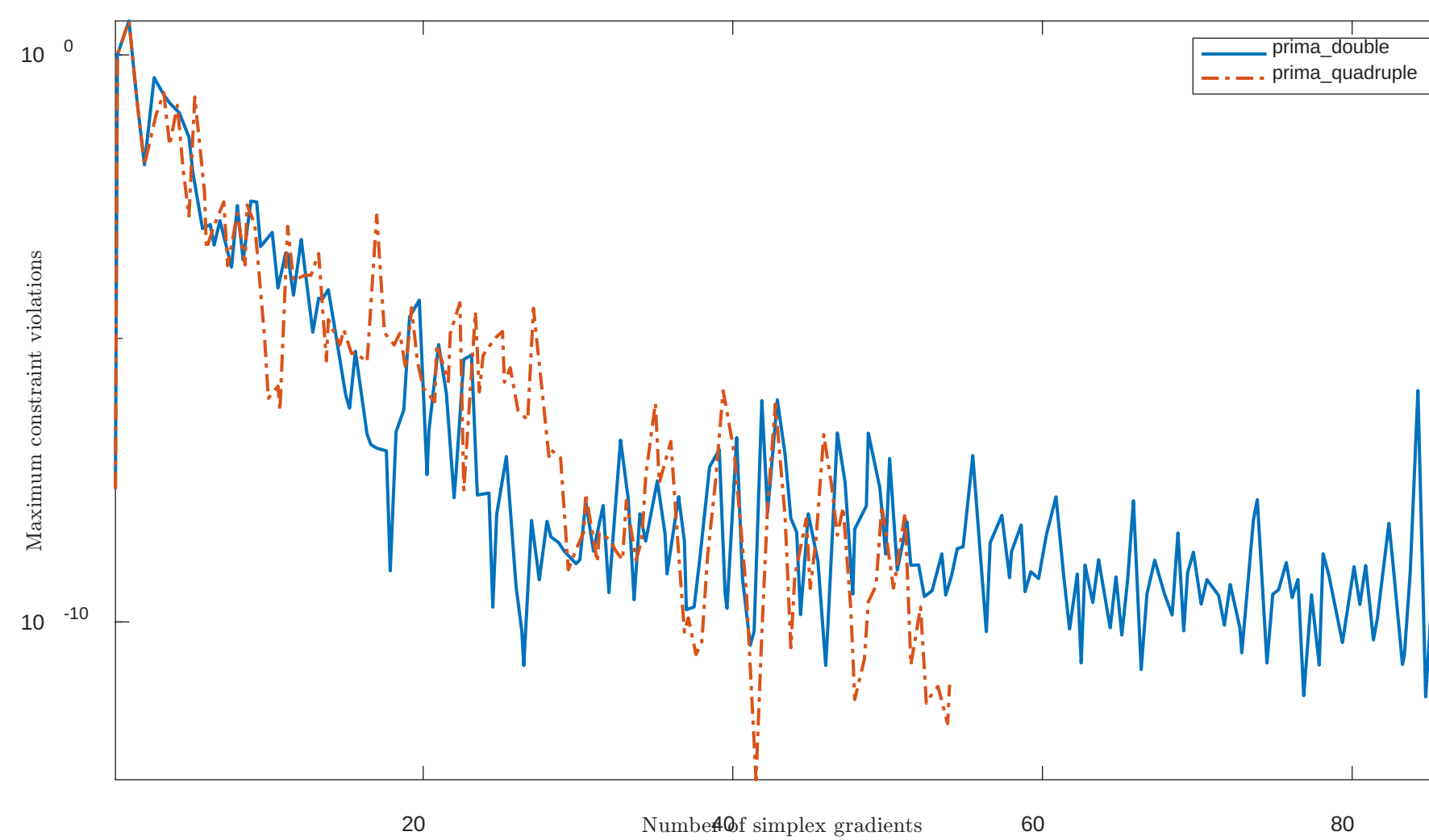
Solving "HS56" with "plain" feature
