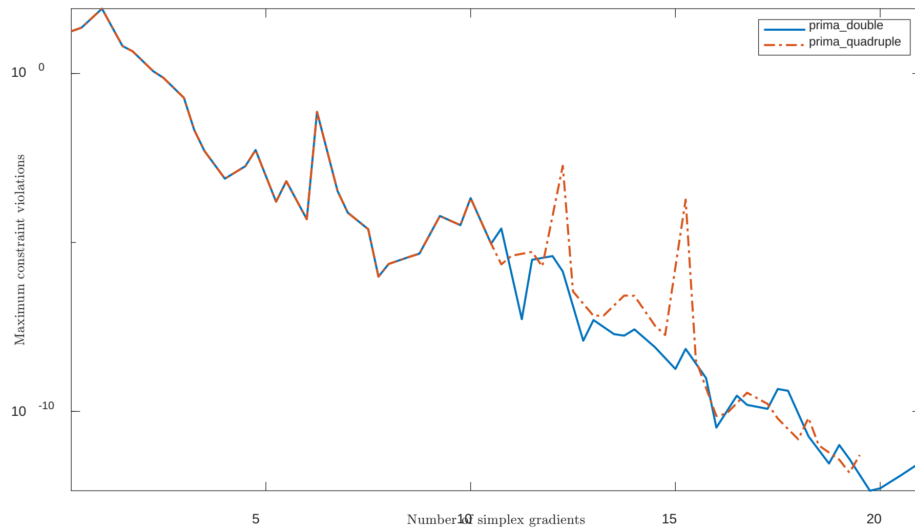
Solving "HS60" with "plain" feature
