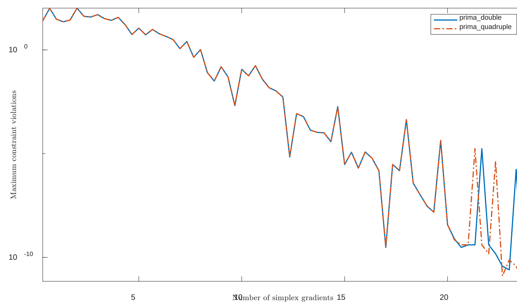
Solving "HS7" with "plain" feature
