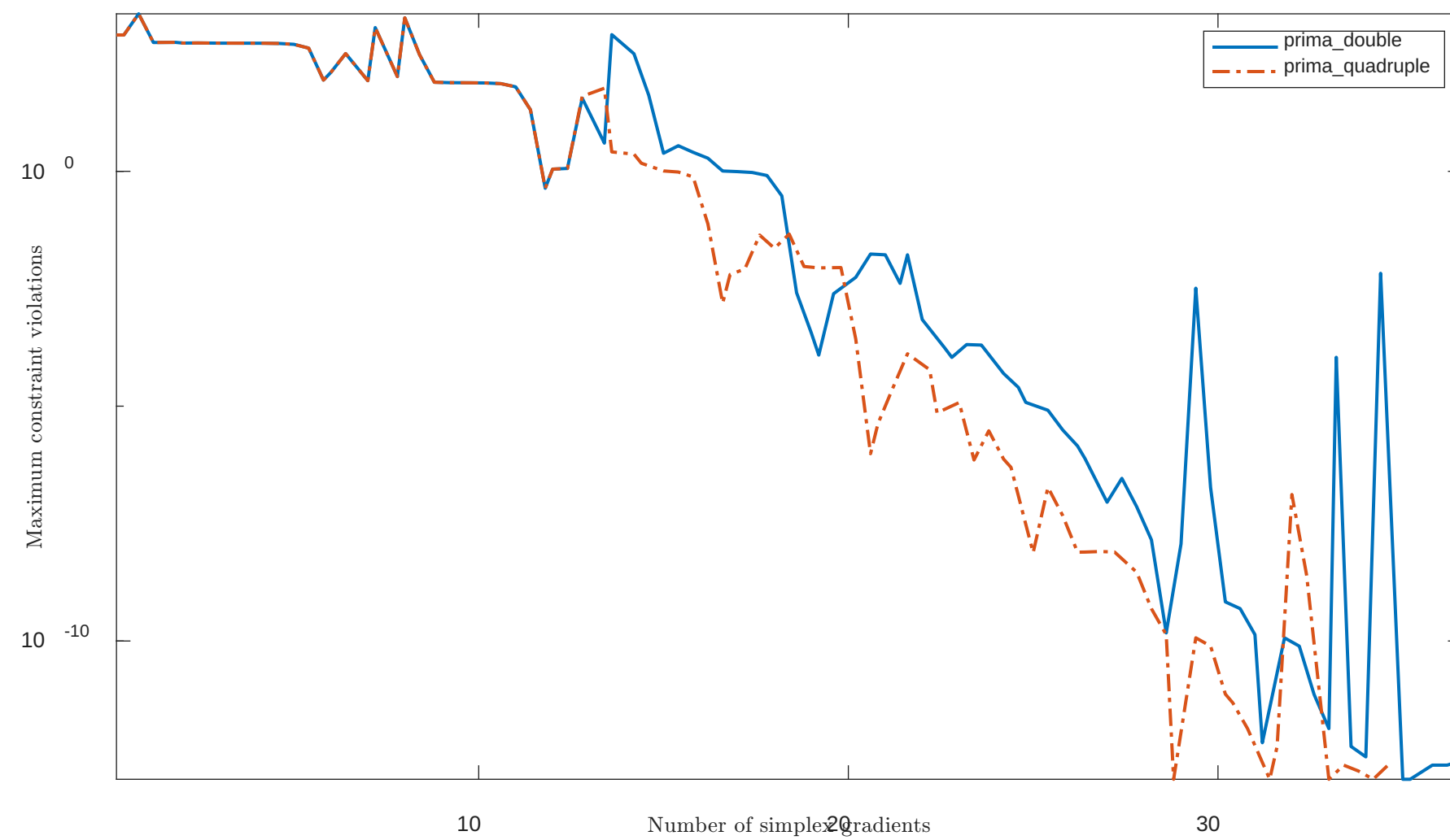
Solving "HS74" with "plain" feature
